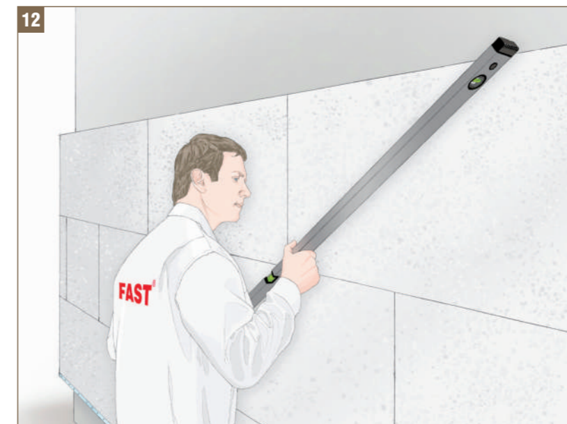
Fig. 12 - Checking board flushness after fixing © FAST 2008
