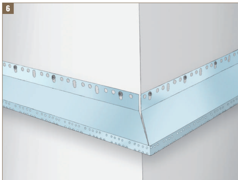
Fig. 6 - Mounting first starter track at the corner of the building © FAST 2008
